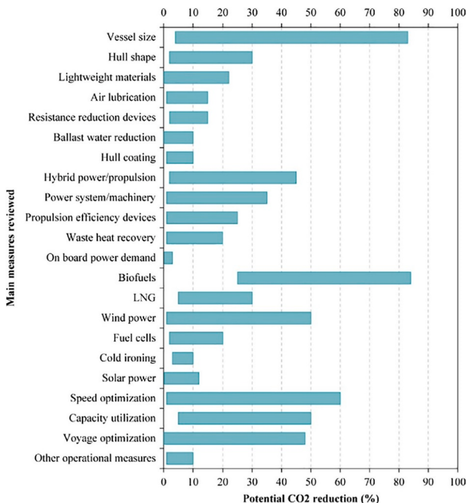
Fig. 29. Potential CO 2 reduction from an array of technical and operational solutions [168,237].
